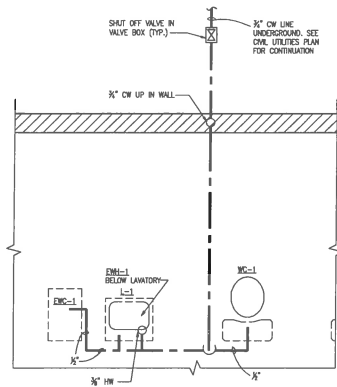
2 TYPICAL RESTROOM WATER PLAN P201 SCALE: 1/2" = 1' - 0"
