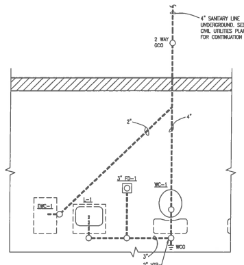
3 TYPICAL RESTROOM SANITARY PLAN P201 SCALE: 1/2" = 1' - 0"
