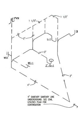
4 TYPICAL SANITARY RISER DIAGRAM P201 SCALE: NOT TO SCALE
