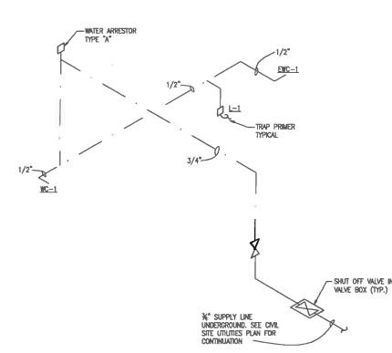
5 TYPICAL WATER RISER DIAGRAM P201 SCALE: NOT TO SCALE
